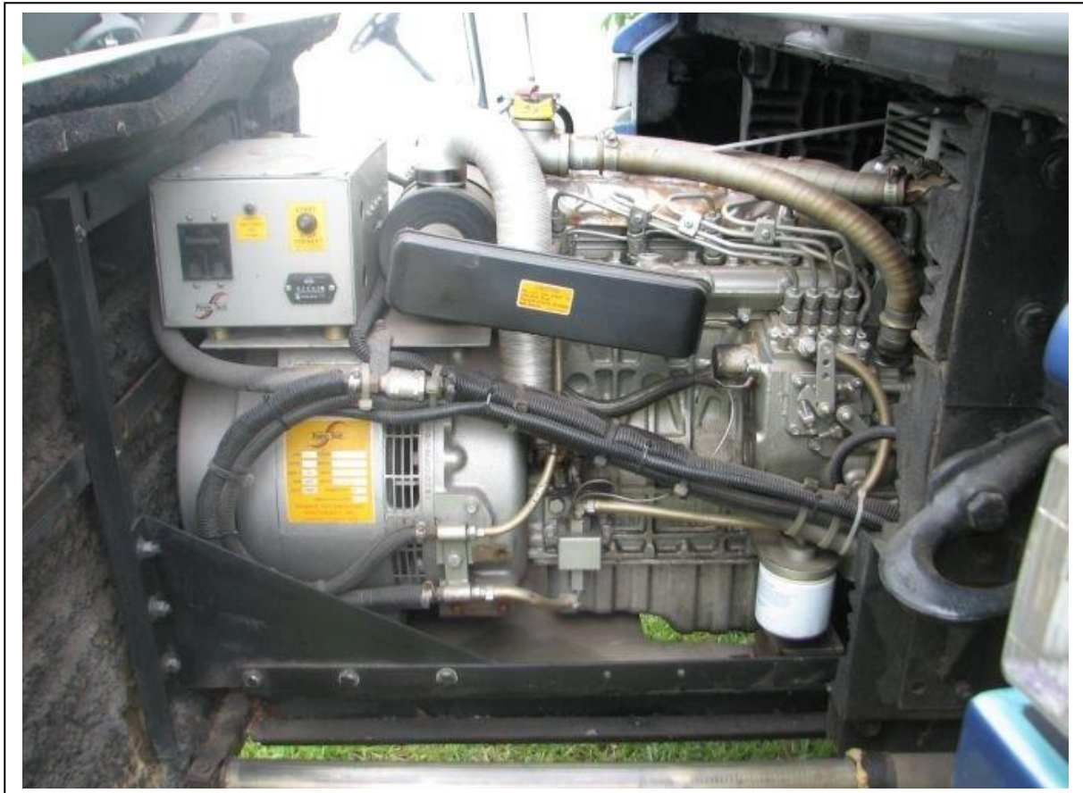
Photo # 14 Description: Powertech generator
